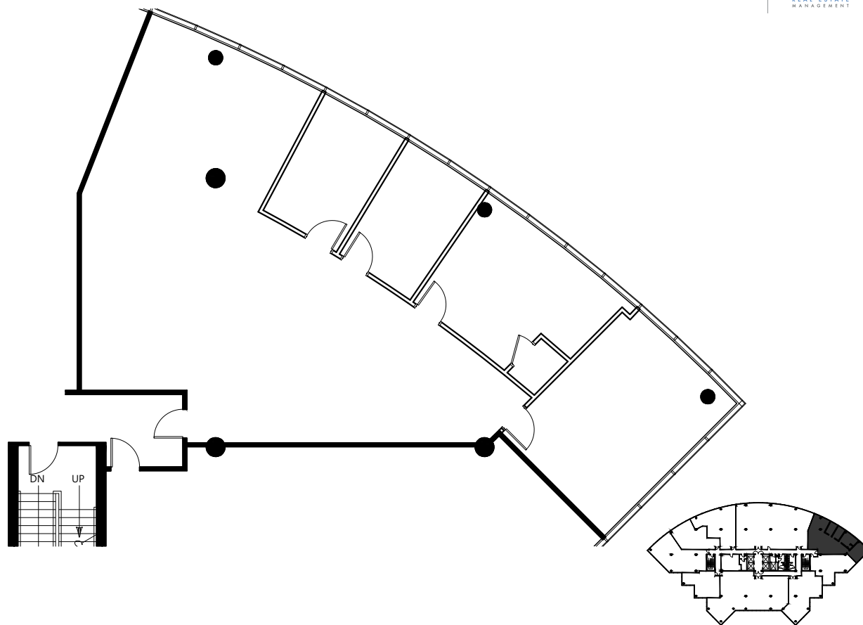
Key Plan
