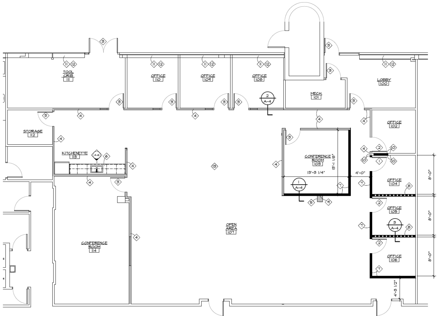
FLOOR PLAN 3/16" = 1'-0"
