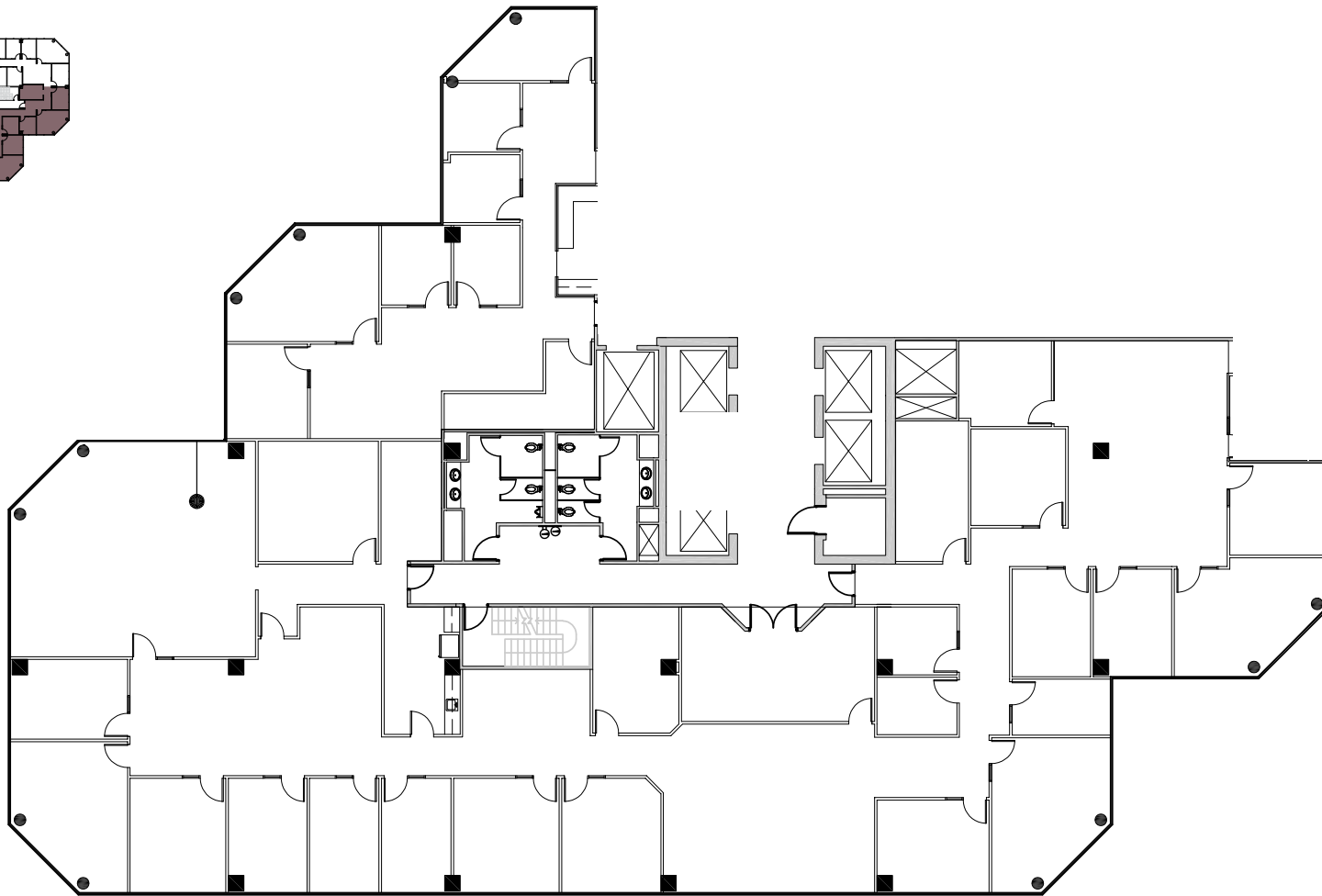
FLOOR PLATE
