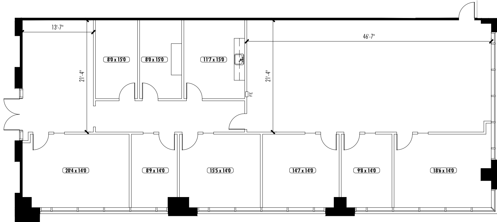
Key Plan
