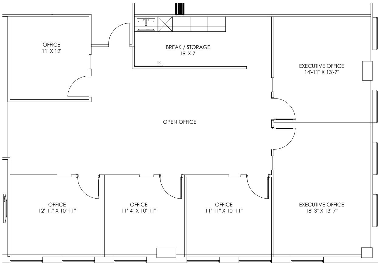
KEY PLAN
