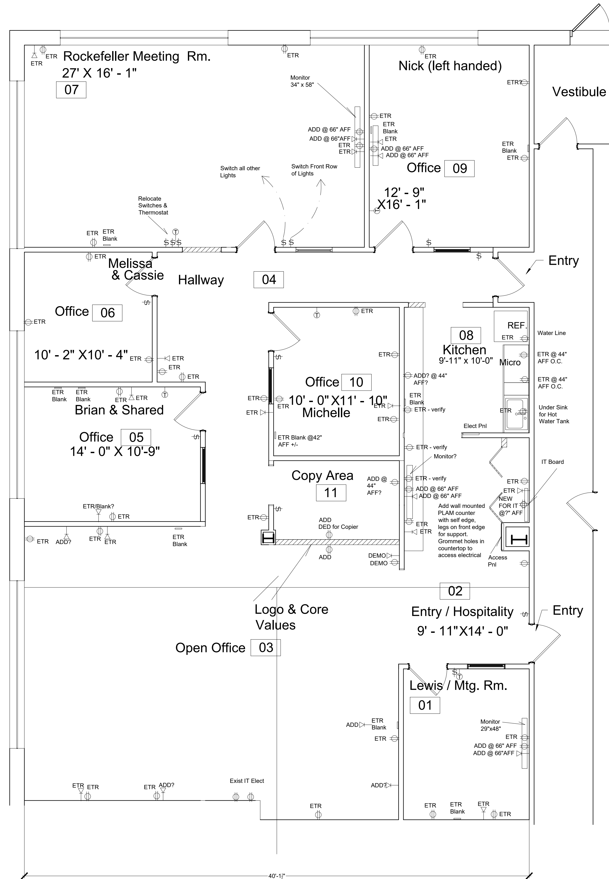
ELECTRICAL PLAN
