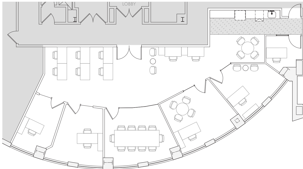
HYPOTHETICAL FURNITURE PLAN
