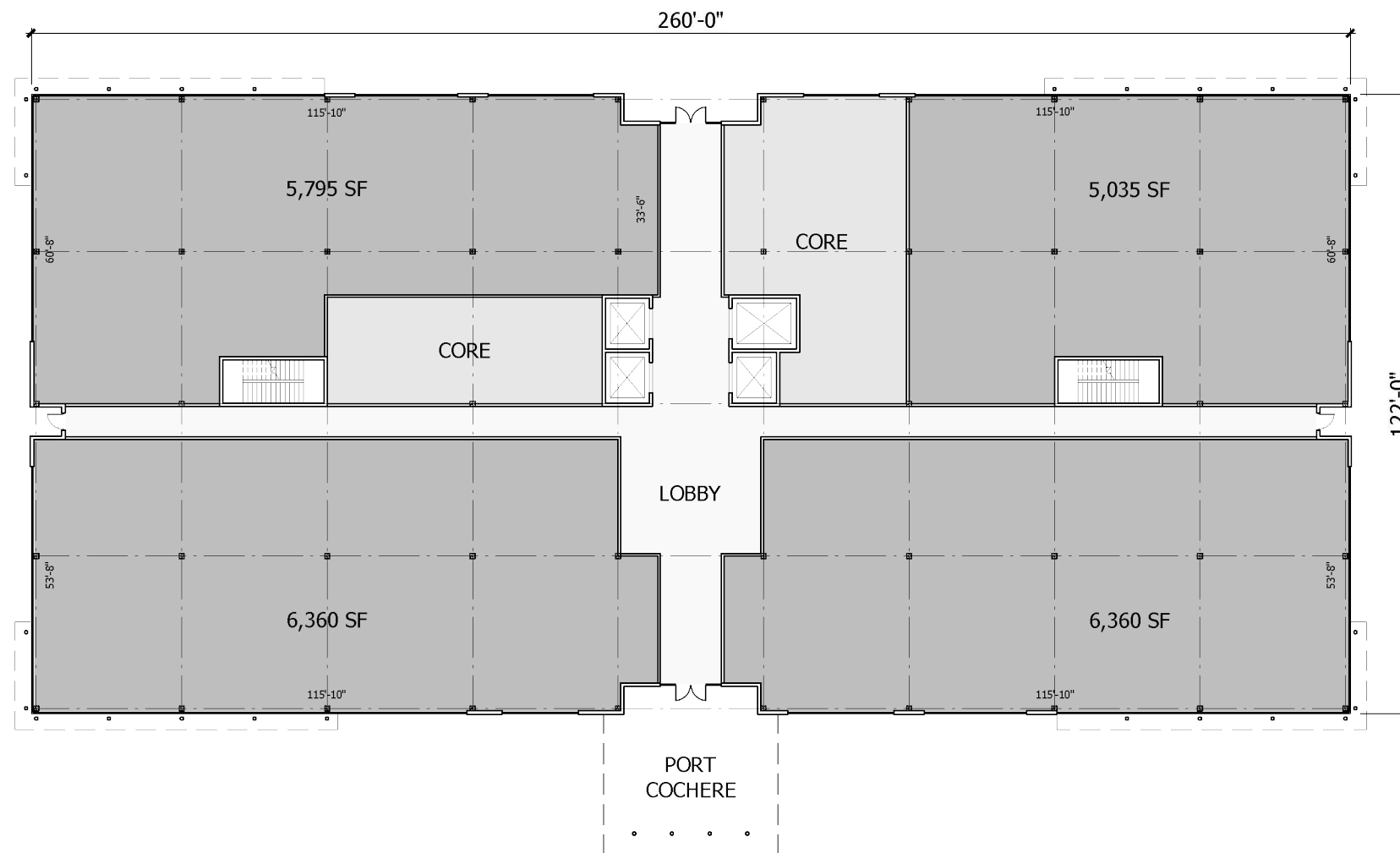
1 GROUND FLOOR PLAN SCALE: 1/32" = 1'-0"
