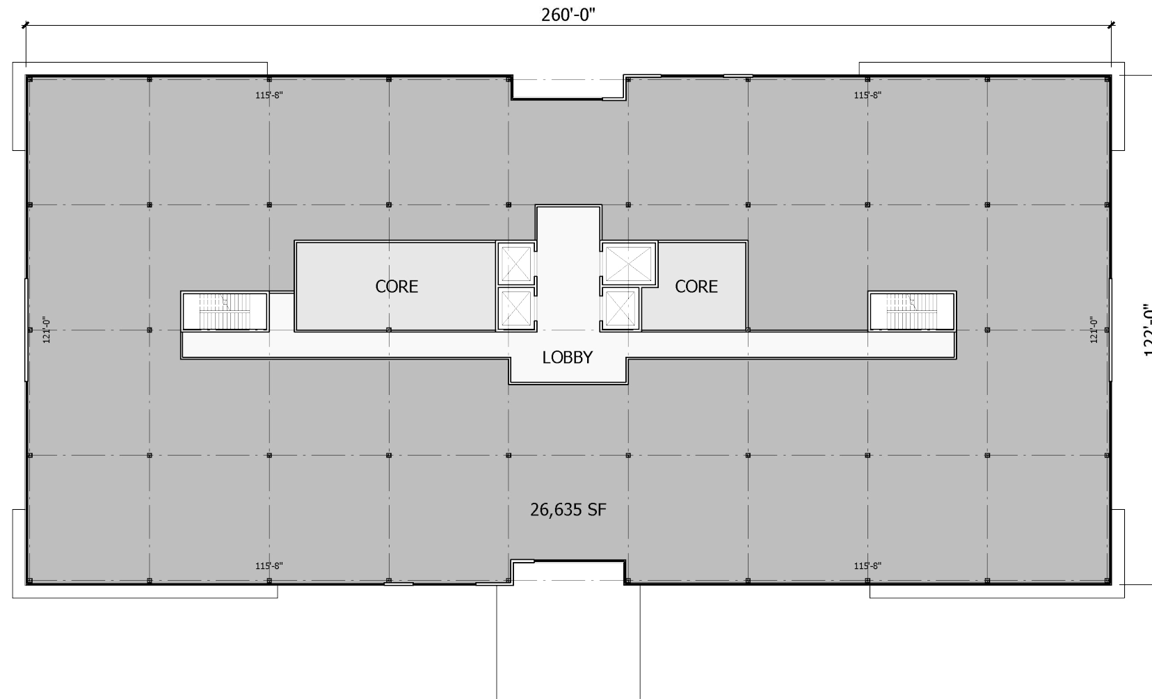
1 SECOND FLOOR PLAN SCALE: 1/32" = 1'-0"
